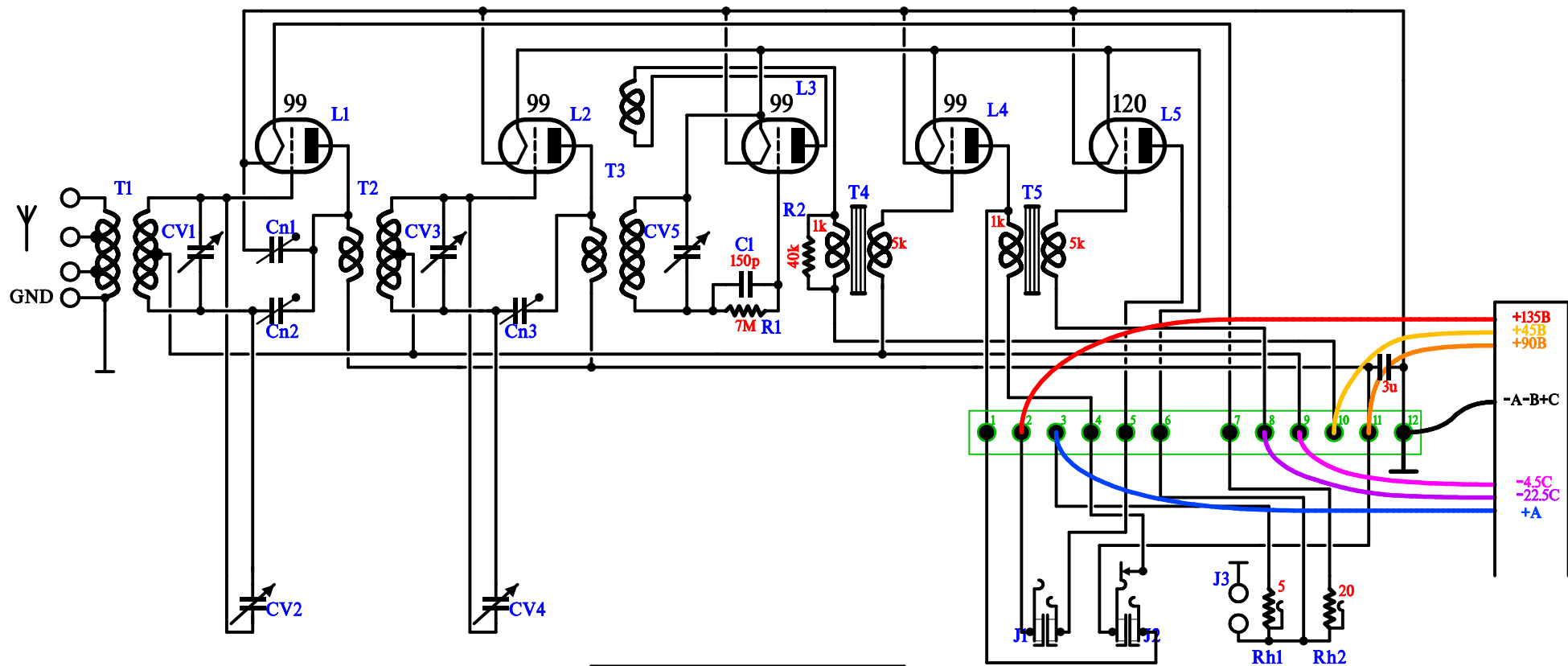
RCA model Radiola 20
