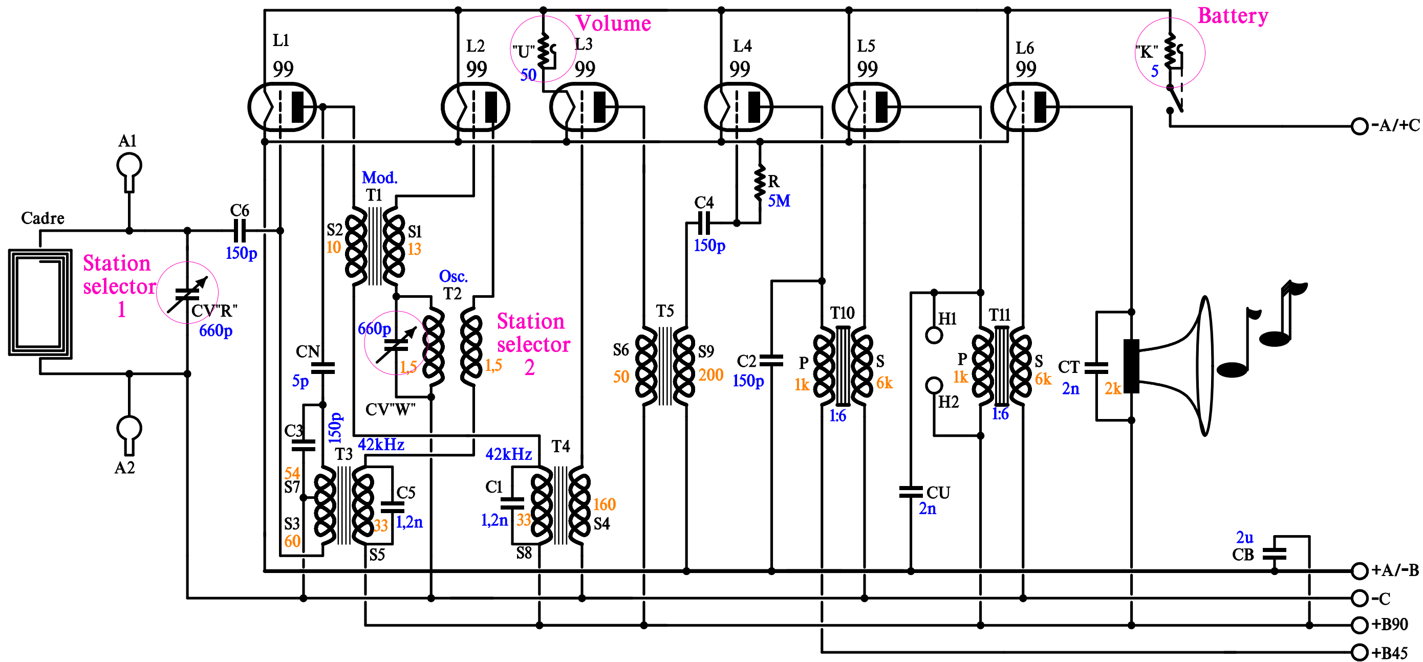
RCA type Radiola 26
